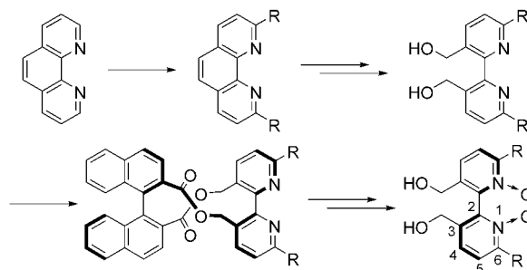
Scheme 1. Previous synthetic route to axially chiral bipyridine N,N' -dioxides.
