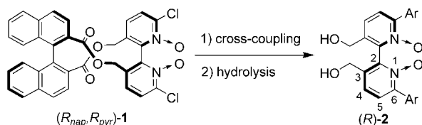
Scheme 2. New approach to axially chiral bipyridine N,N' -dioxides ( R )- 2 bearing various aromatic substituents at the 6 and 6' positions.
