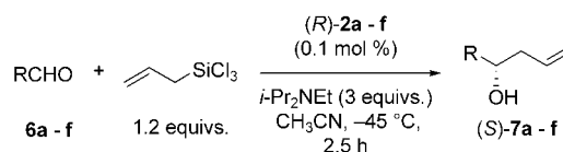
Scheme 4. Asymmetric allylation of aldehydes with allyl(trichloro)silane; \text{R} = 4\text{-MeOC}_6\text{H}_4 ( 6a ), 4\text{-CF}_3\text{C}_6\text{H}_4 ( 6b ), Ph ( 6c ), 2\text{-MeC}_6\text{H}_4 ( 6d ), 2-furyl ( 6e ), ( E )- \text{PhCH=CH} ( 6f ).
