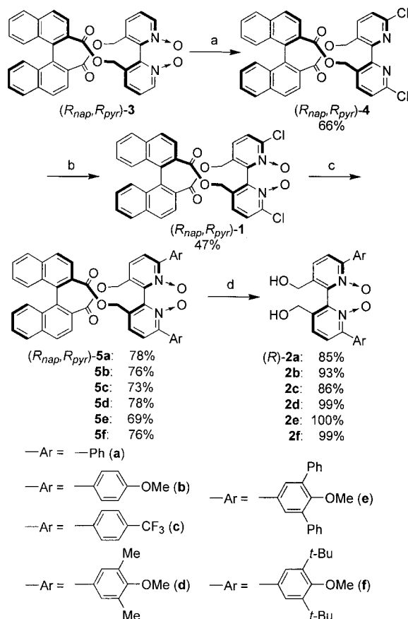
Scheme 3. Preparation of axially chiral bipyridine N,N' -dioxides ( R )- 2 ; a) \text{POCl}_3 (3 equivs.), \text{NaCl} (20 equivs.), DMF, 60^\circ\text{C} , 2 h; b) \text{H}_2\text{NCONH}_2 \cdot \text{H}_2\text{O}_2 (3.1 equivs.), (\text{CF}_3\text{CO})_2\text{O} (3 equivs.), \text{CH}_3\text{CN}/\text{CH}_2\text{Cl}_2 , 0^\circ\text{C} to rt, 3 h, ( \times 3 ); c) \text{ArMgBr} (3 equivs.), \text{PdCl}_2(\text{dppf}) (5 mol %), THF, -15^\circ\text{C} , 1 h; d) 6 N \text{NaOH} , MeOH.
